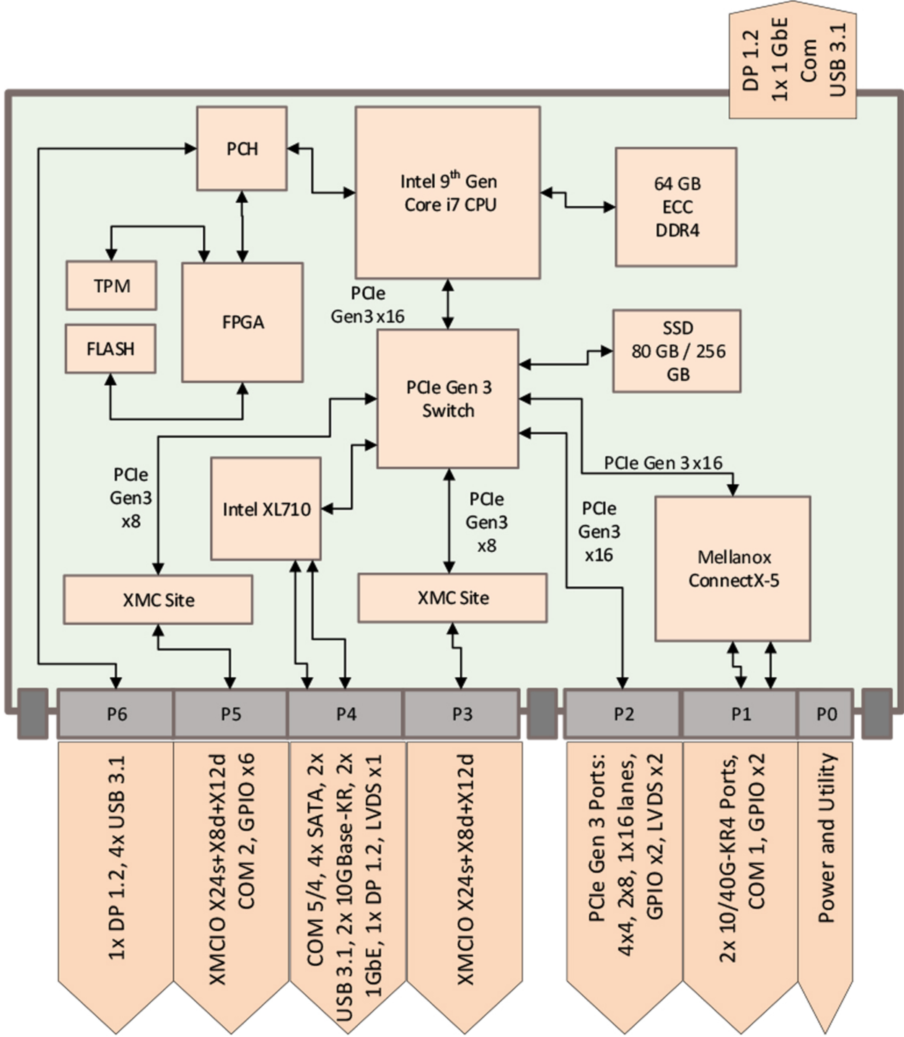
Block diagram (Non-SOSA)
