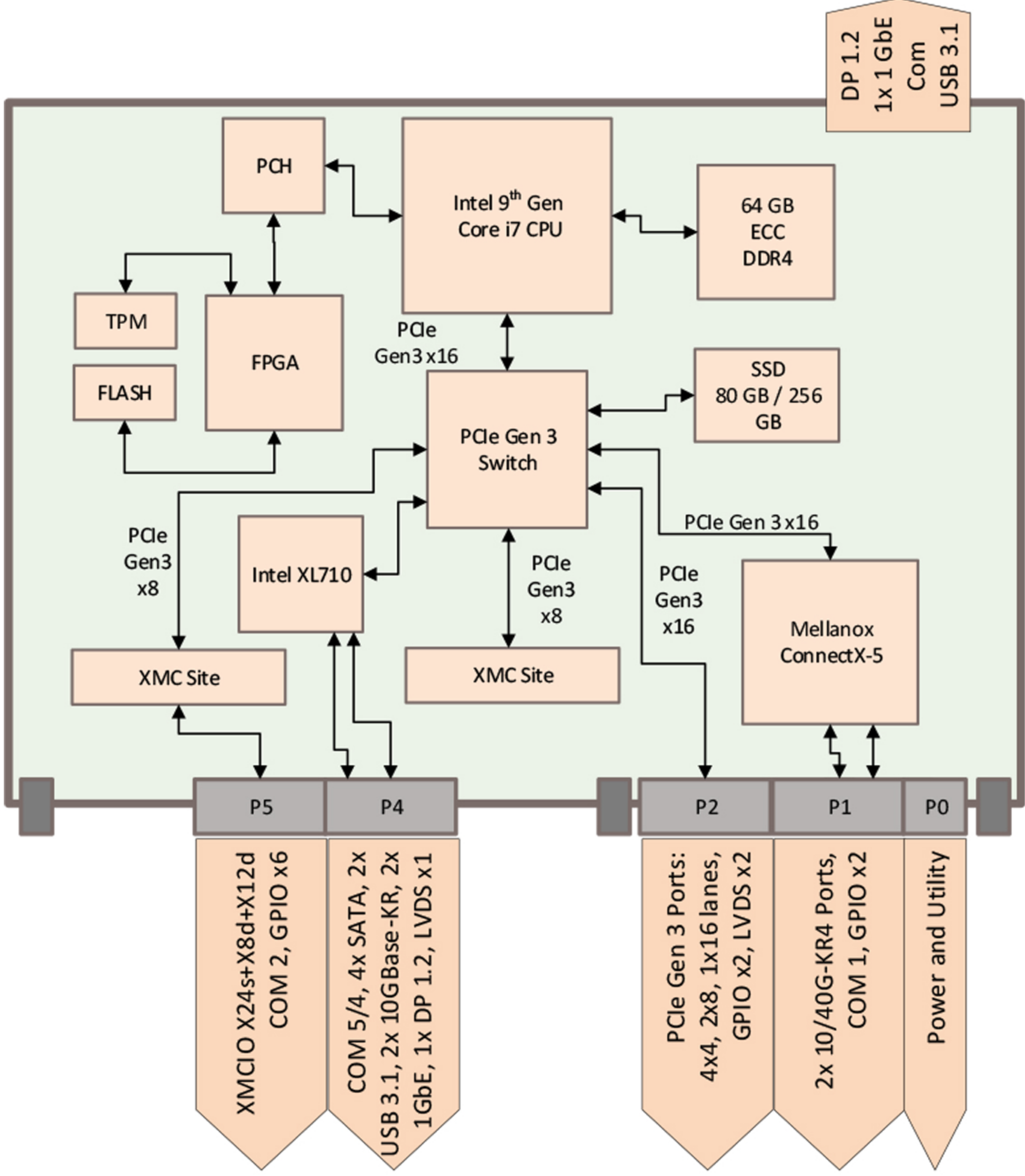
Block diagram (SOSA-Aligned)
